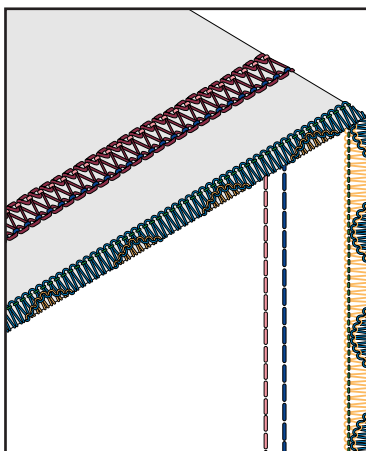
6-Thread Stitch Cover Stitch Narrow Left w/ 3-Thread Rolled Wave
