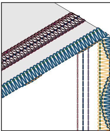
7-Thread Stitch Triple Cover Stitch w/ 3-Thread Wave Stitch
