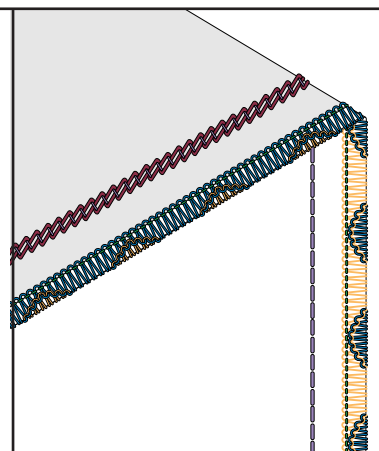
5-Thread Stitch Right Chain Stitch w/3-Thread Rolled Wave
